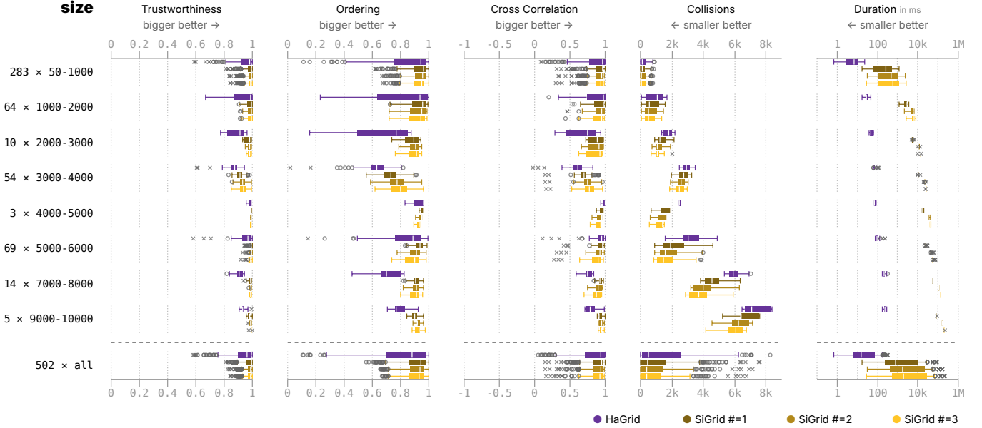
Fig. 5: Comparison of Hagrid and SiGrid (with 1, 2, or 3 SBR iterations). Datasets are binned by their number of points. Except for the 4000–5000 bin, SiGrid leads to an improvement in trustworthiness, ordering, cross-correlation, and collisions at the cost of increased runtime. (Hagrid parameters are level: min_level, ensure_whitespace: 0; SBR parameters are iterations: 1, 2, or 3, number_of_sectors: 8). Hagrid needs to use a finer grid for datasets with N > 4096 to be able to assign all points, which leads to 16384 grid cells.
