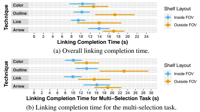
Figure 4: Completion time measures using mean and 95% CIs.
