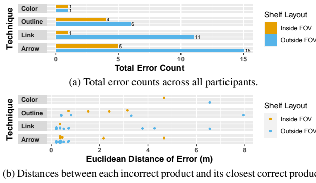
Figure 5: Error measures for the single- and multi-selection task.
