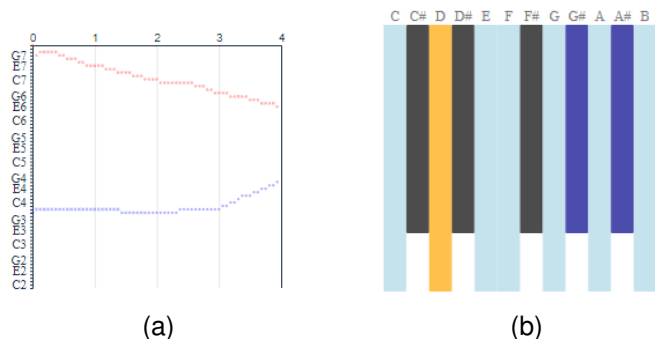
Fig. 4: Two filters allow steering model sampling (a) by pitch range per step and (b) by allowed chroma. In this example, (a) we narrow the range toward the end to get a controlled and more concentrated ending. Also, (b) we allow any chroma but C#, D#, and F# (gray), while we select D as our root note (orange) to look for samples that are highly related to the D minor key using our other visualizations, as Brachtel did in his commissioned work.
