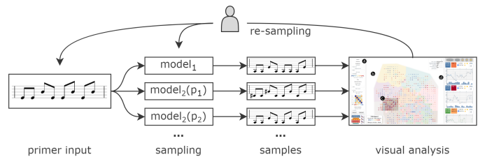
Fig. 2: In visual parameter space analysis [75], the models’ output gets sampled for different parameterizations ( p_i ) and then visualized. Iterative re-sampling allows the analyst to further explore interesting areas of the parameter space. This analysis provides insights into the model’s behavior and enables more effective usage.
